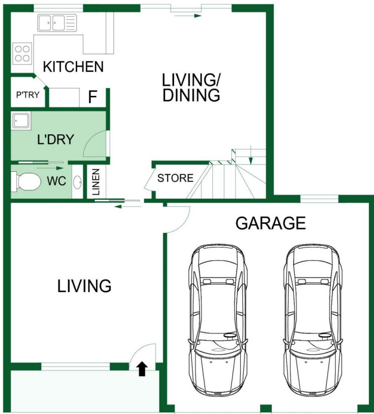
LOWER FLOOR
