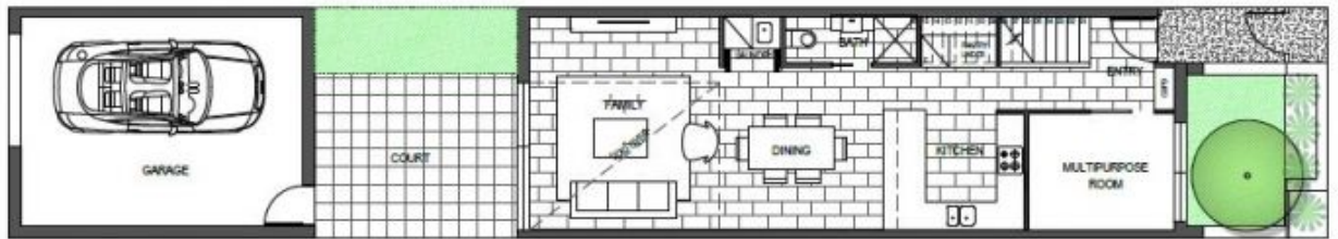
LOWER FLOOR PLAN
